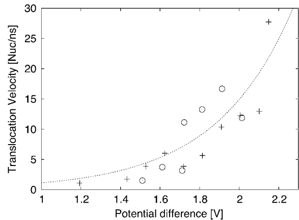
FIGURE 11 Translocation speed in nucleotides per nano second plotted versus the potential difference across the membrane. Both translocations in an H/OH-CNT (+) and a naked CNT (○) are plotted. An exponential is fitted to the data.
