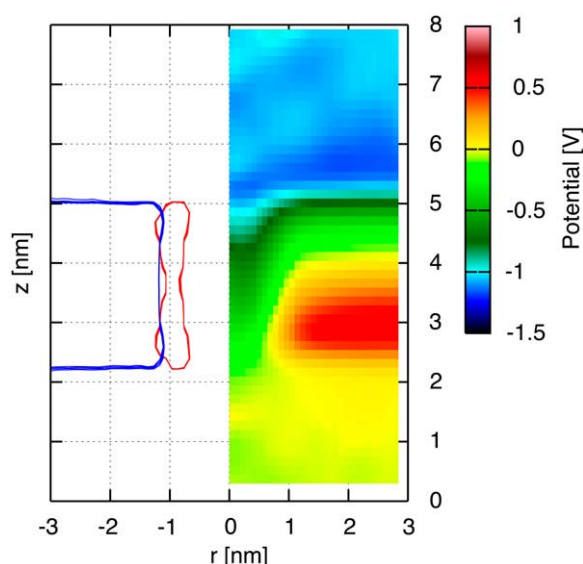
FIGURE 7 CNT in a dodecane membrane. Averaged electrostatic potential map (right), and the corresponding radially averaged density profile for the dodecane (blue) and the CNT (red) molecules on the (r, z) plane. A potential difference of 0.955 V acts across the dodecane membrane.
