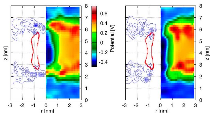
FIGURE 3 Potential maps and density profiles on the ( r , z )-plane for a naked CNT (left panel) and a decorated H/OH CNT (right panel) acting as nanopores in a DMPC lipid bilayer in the absence of an imposed electrostatic transmembrane potential difference. The electrostatic potential map (right half in each figure), and density profile (left half in each figure) are plotted to demonstrate correlations between the distribution of the lipid heads and the resulting potential. The density profiles indicate the CNT-carbon atoms (red) and the DMPC-nitrogen atoms (blue). There is no electrostatic potential difference acting across the membrane. Zones of high electrostatic potential protrude slightly into the pore area for the decorated CNT (left), whereas for the case of a naked CNT (right) they form a barrier across the entrance of the tube.
