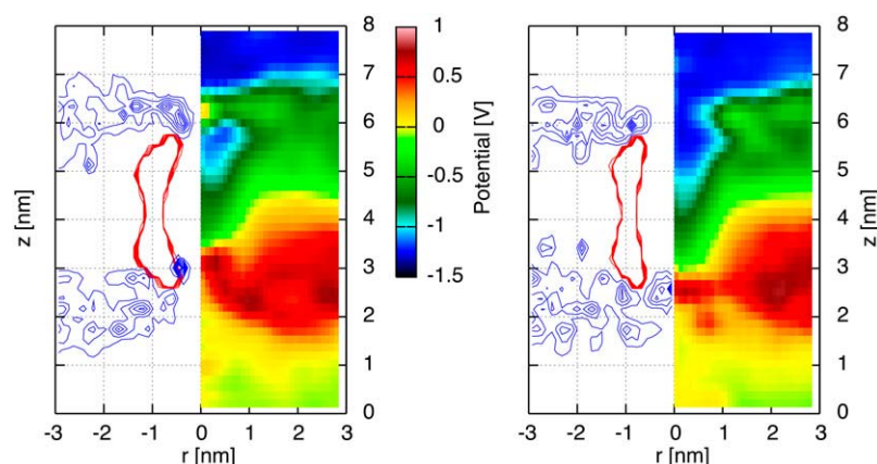
FIGURE 8 A naked CNT (left panel) and a decorated CNT (right panel) in a DMPC membrane subject to a electrostatic potential difference of 1.05 V. Radially averaged electrostatic potential map (right half of each figure) and density profile (left side of each figure) on the (r, z) plane of the nitrogen of the DMPC (blue) and the CNT (red) molecules.
